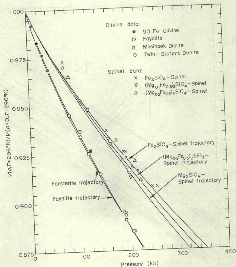
FIG. 8. Comparison of the calculated pressure-volume relation of olivine with experimental compression data. The solid lines are the present work, independent of compression data points. The isothermal compression data of olivine are due to Bridgman (●) and to Takahashi (○). The shock compression data are due to McQueen, Marsh, & Fritz for Mooihoek dunite (□) and Twin-Sisters dunite (◇). The isothermal compression data of olivine-transformed spinels are due to Mao et al. (1969), and the solid lines are the calculated pressure-volume relation for the olivine-transformed spinels in the \text{Mg}_2\text{SiO}_4 - \text{Fe}_2\text{SiO}_4 series established by Chung (1971b).
